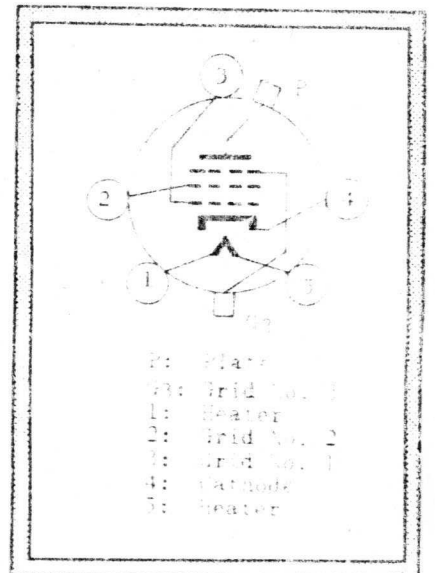
TERMINAL CONNECTIONS
