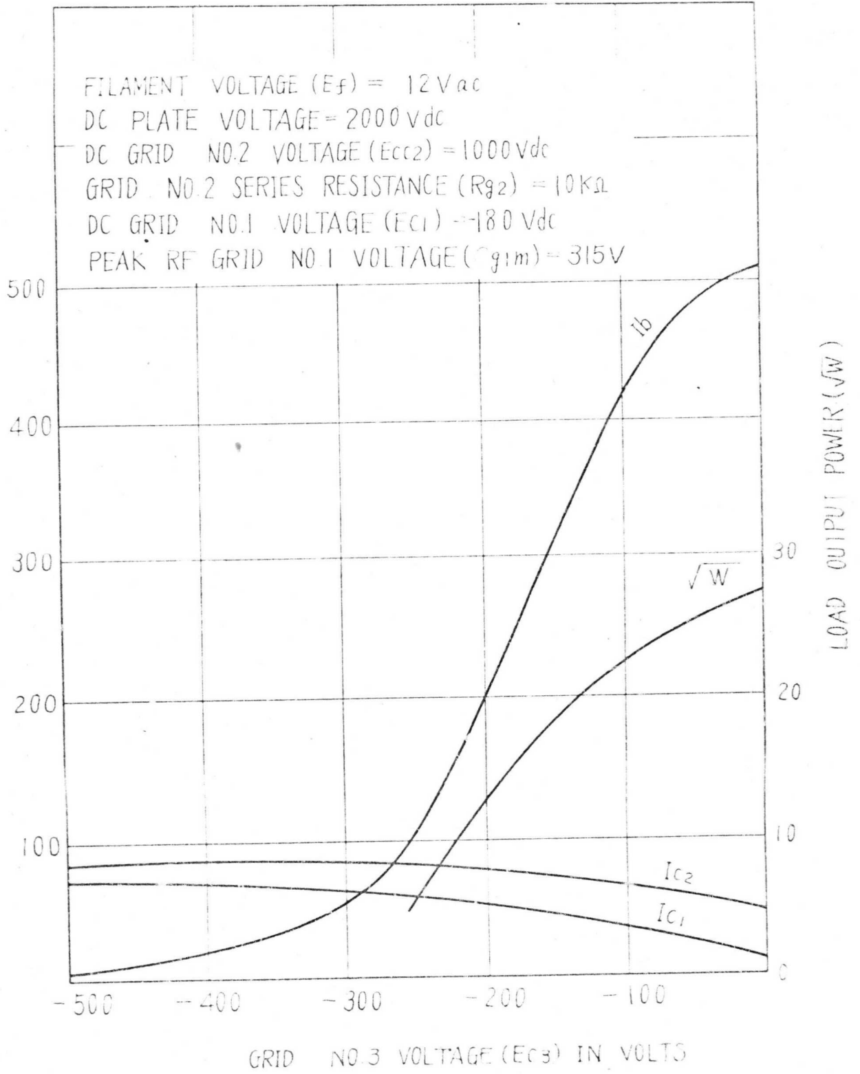
P250A GRID NO. 3 MODULATED CHARACTERISTICS
