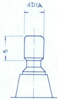
DETAIL OF COLLECTOR CAP
