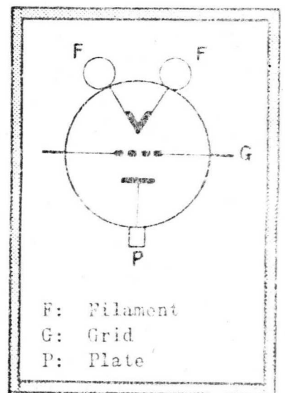
TERMINAL CONNECTIONS
