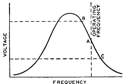
Fig. 29—Resonance curve of a tuned circuit showing desired operating range for frequency-modulation converter.
