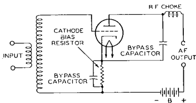
Fig. 26—Grid-bias detector circuit.
