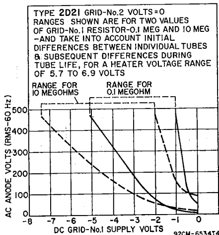
Operational Range of Critical Grid-No. 1 Voltage.
