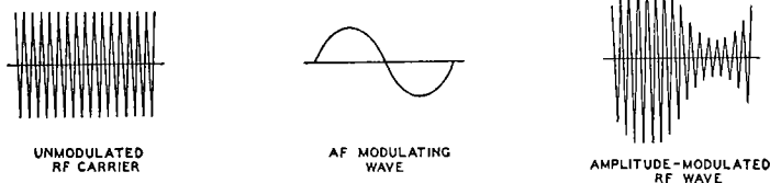
Fig. 21—Waveforms showing effect of amplitude modulation on an rf wave.
