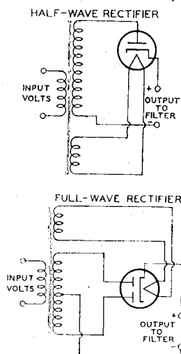
Fig. 18—Half-wave and full-wave rectifier circuits.
