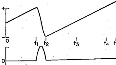
Fig. 87—Yoke-current (upper) and switch-voltage (lower) waveforms when switch is closed at t_2 .
