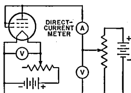
Fig. 129—Fundamental circuit of an emission tester
