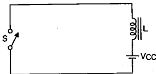
Fig. 85—Simplest form of deflection circuit.
