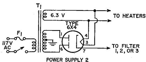
POWER SUPPLY 2
