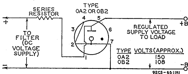
Typical circuit to provide regulated supply voltage of approximately 150 or 108 volts to load. Removal of tube from socket removes voltage from load.
