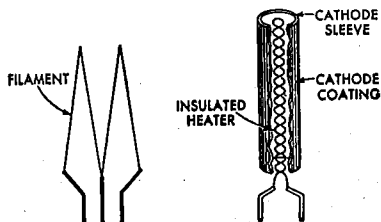
Fig. 2—Indirectly heated heater-cathode.
