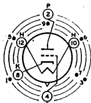
12AQ INDEX-LARGE LUG ●●SHORT PIN-IC
