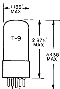
T-9 GLASS BULB INTERMEDIATE SHELL 8 PIN OCTAL B8-6 OUTLINE DRAWING JEDEC 9-15
