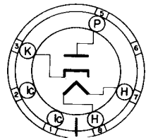
BOTTOM VIEW • INTERMEDIATE SHELL OR SHORT INTERMEDIATE SHELL 8 PIN OCTAL 4CG
