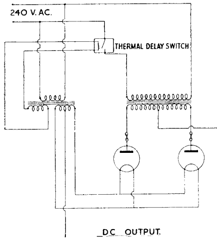
A typical H.T. rectifier circuit using a thermal delay switch in the primary of the H.T. transformer.
