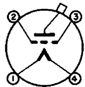
Terminal Layout
